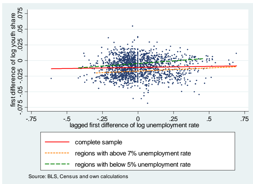
Figure 6: First difference of log youth share and lagged first difference of unemployment rate, state level data, 1973-2005
