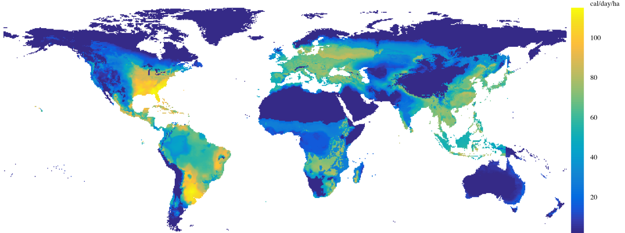
FIGURE 2: The Global Distribution of the Potential Caloric Return of Native Crops Before AD 1500. Notes: This figure depicts the worldwide distribution of daily crop yields, as measured by the ratio of total crop yields to crop growth cycles, for crops that were native to a location before AD 1500. Higher (lower) daily crop yield values are indicated by pixels closer to the yellow (blue) end of the color spectrum. Source: Based on data from Galor and Özak (2016).
