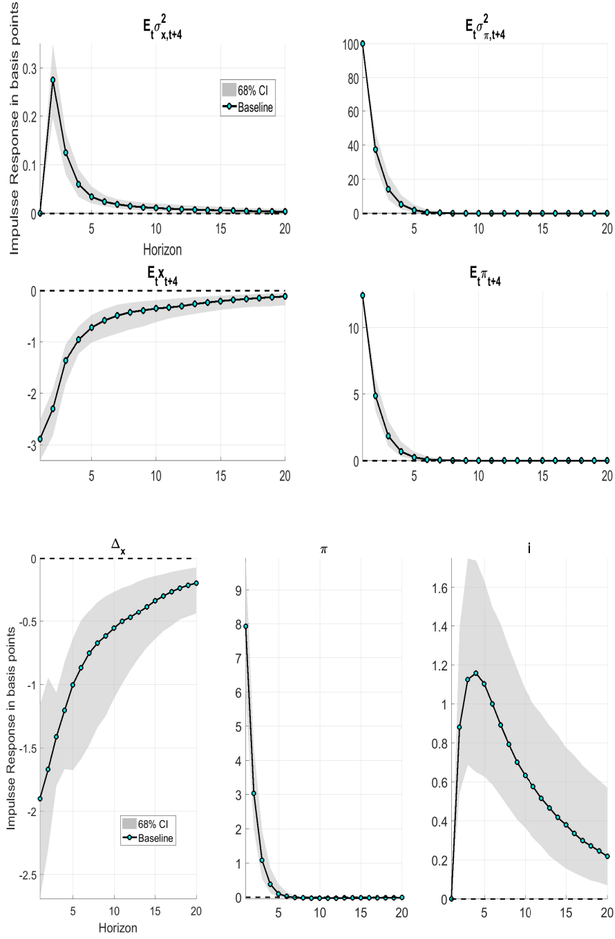
Figure 5: Impulse Responses of Perceived Uncertainty about x_{t+4} , \pi_{t+4} , Expectations of x_{t+4} , \pi_{t+4} , Output Gap ( \Delta_x ), Inflation ( \pi ) and the nominal interest rate ( i ) for a 1% shock to perceived uncertainty about \pi_{t+4} . Shaded area denotes 68 % credible interval.
