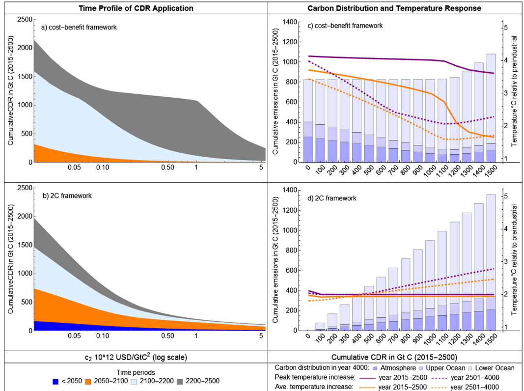
Figure 2. CDR time profile and cumulative emissions in CC16. The left panel shows the time profile of CDR utilization as function of c_2 , the slope of the marginal CDR cost curve for the different mitigation frameworks (CBA and 2C in (a) and (b), respectively). The right panel shows the cumulative emissions (from 2015 until 2500) as function of the cumulative amount of CDR for the different mitigation frameworks (CBA and 2C in (c) and (d), respectively). The right panel also includes information about the distribution of the carbon emissions among the different carbon reservoirs in the year 4000 and about peak and average temperature for the period 2015–2500 and 2501 until 4000.
