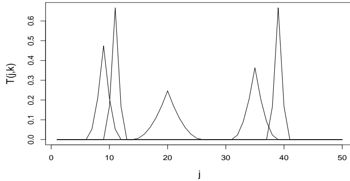
Figure 1: T_{jk} for p = 50 and 5 different k
