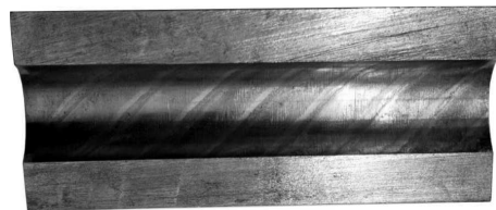
Figure 2: Effect of spiralling on the bore hole wall
