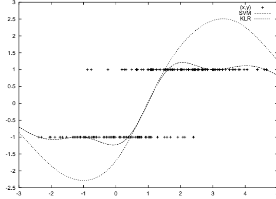
Figure 1: One-dimensional comparison of SVM and KLR predictions. Negatives examples are drawn from N(0,1) (dots at y=-1 ), positive examples from N(2,1) (dots at y=1 ). Both methods find the class border at x=1 , but the SVM prediction is essentially constant for y outside [-1,1] . KLR correctly estimates higher confidences for points nearer to class centers.
