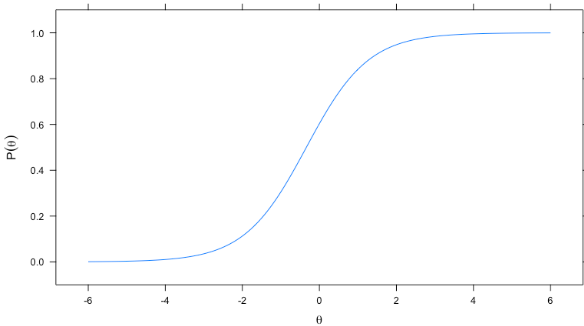
Figure A1: Item Characteristic Curve (Item 2)
