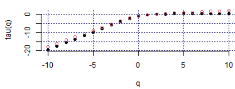
Mass exponent (MYS_BURSA, c1)
