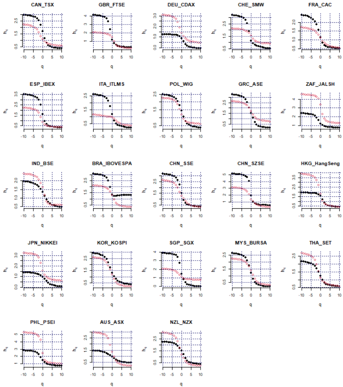
Fig. 6: Generalised Hurst exponent for each market index, from q = -10 to 10 , for pre- (black) and post-(red) level 1 (C1) stay-at-home policy recommendation.
