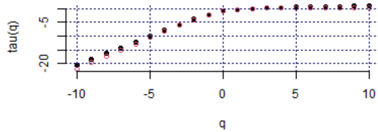
Mass exponent (USA_NASDAQ, c2)
