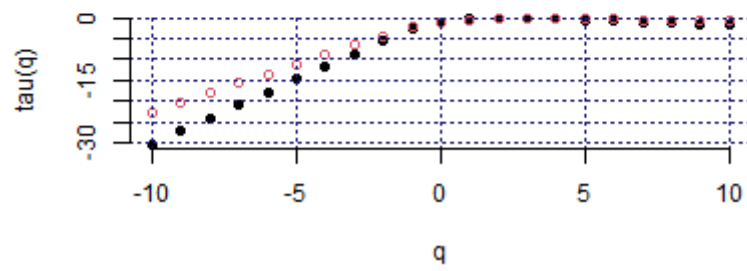
Mass exponent (ITA_ITLMS, c3)
