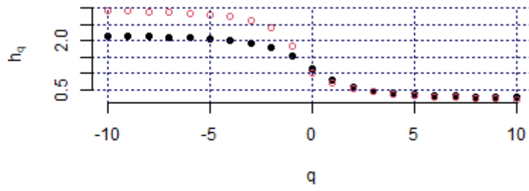
Hurst exponent (CHE_SMW, c2)
