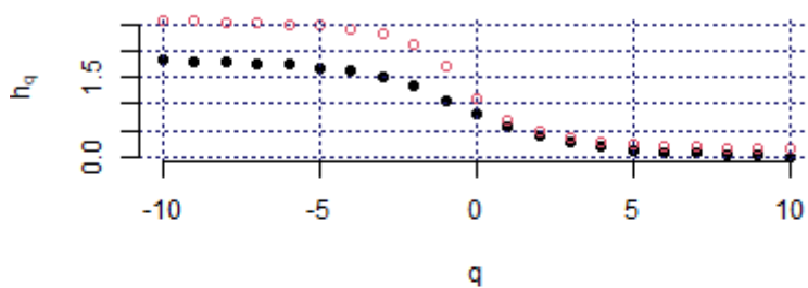
Hurst exponent (THA_SET, c1)
