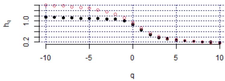
Hurst exponent (FRA_CAC, c1)
