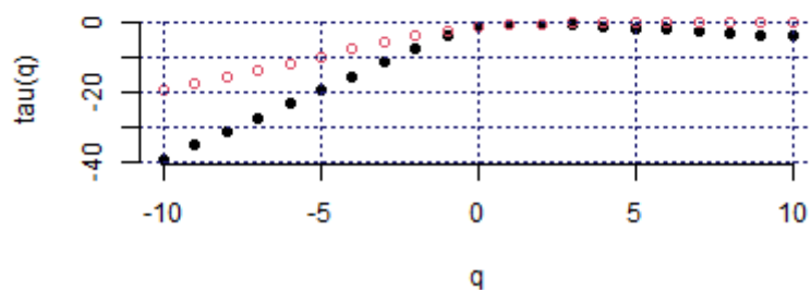
Mass exponent (SGP_SGX, c2)
