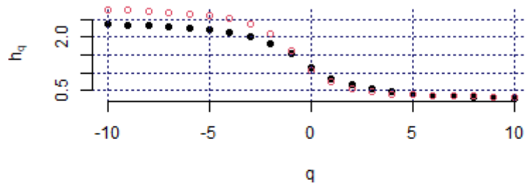
Hurst exponent (BEL_BEL, c2)
