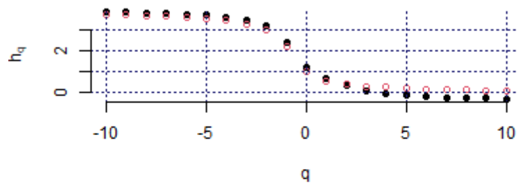
Hurst exponent (SGP_SGX, c1)
