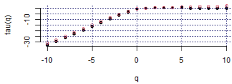
Mass exponent (CHN_SSE, c1)
