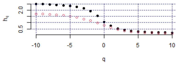
Hurst exponent (NZL_NZX, c2)
