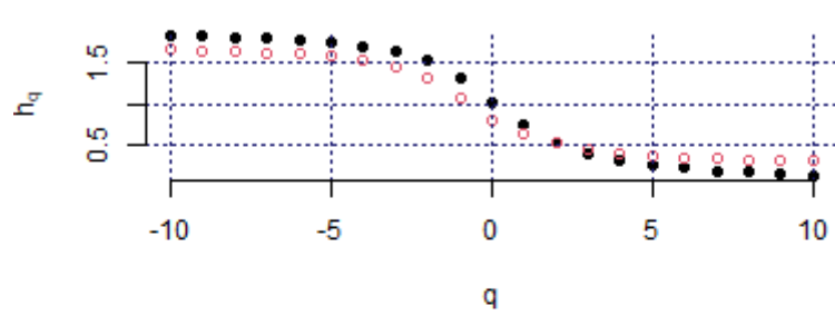
Hurst exponent (MYS_BURSA, c1)
