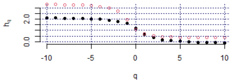
Hurst exponent (CHN_SZSE, c1)
