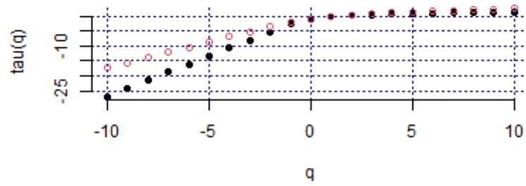
Mass exponent (CAN_TSX, c1)
