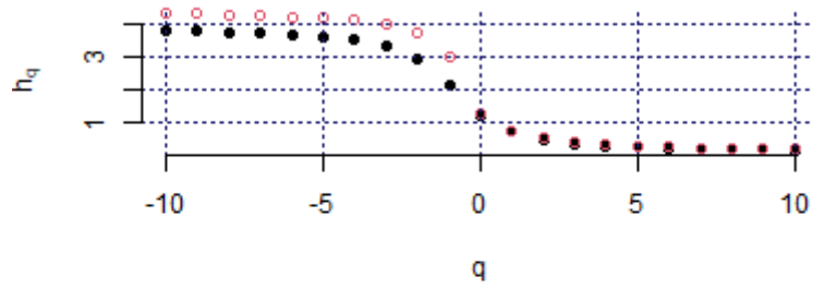
Hurst exponent (CHE_SMW, c1)
