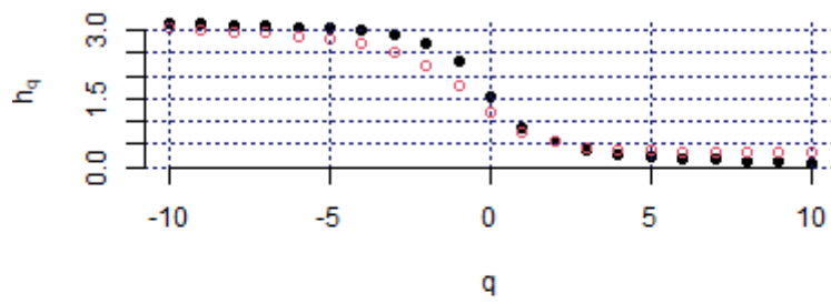
Hurst exponent (CHN_SSE, c1)
