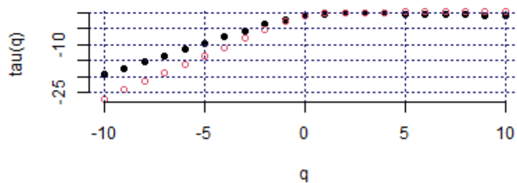
Mass exponent (THA_SET, c1)
