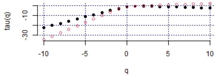
Mass exponent (CHN_SZSE, c1)
