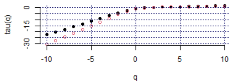
Mass exponent (CHE_SMW, c2)
