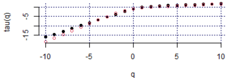
Mass exponent (GRC_ASE, c2)
