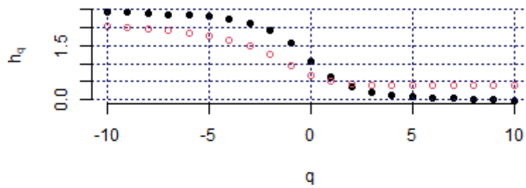
Hurst exponent (ITA_ITLMS, c2)
