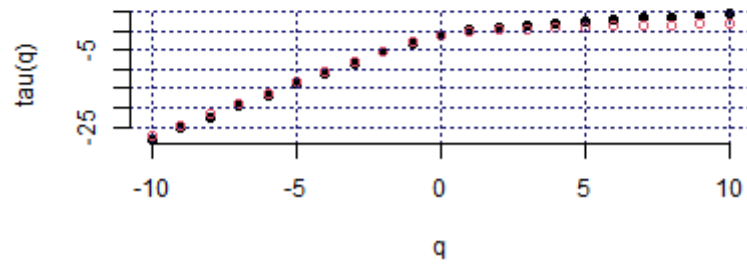
Mass exponent (CHN_SSE, c3)
