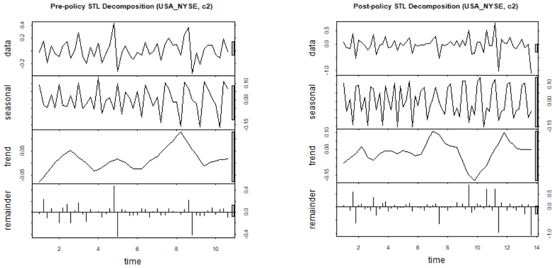
Fig. 1: STL Decomposition for NYSE, Pre (Left) and Post (Right) Policy.
