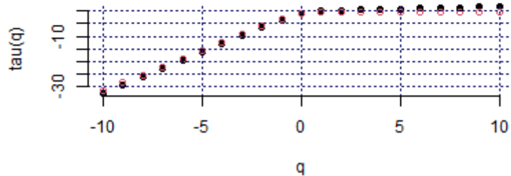
Mass exponent (HKG_HangSeng, c1)
