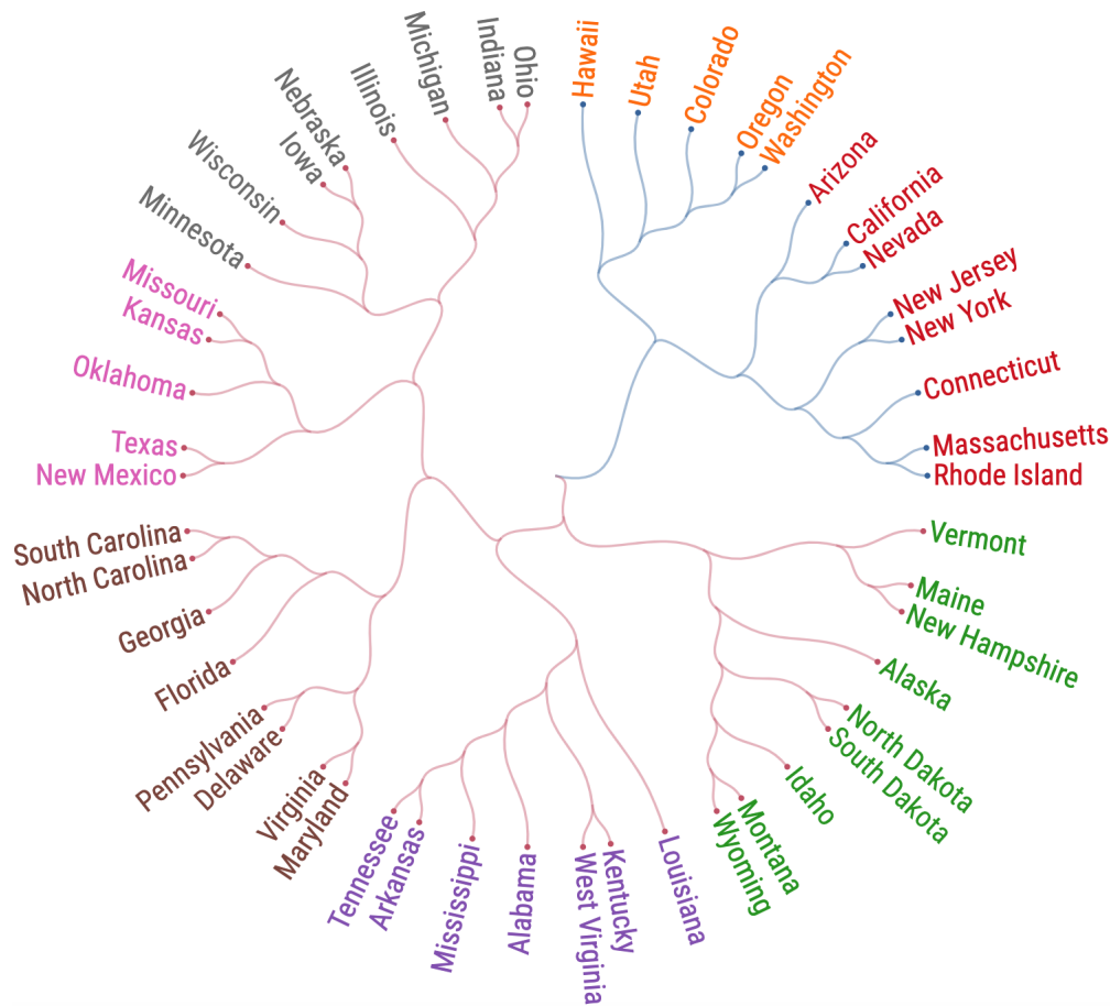
Figure 4: Bottom-up measurement of subnational culture returns sensible clustering of subnational units. Facebook culture vectors drawn from the states of the United States cluster together in an unsupervised manner into traditional regional and cultural groupings. South Carolina bears similarity to North Carolina, Montana to Wyoming, New Jersey to New York, and West Virginia to Kentucky. Similarities are not strictly geographic, with Alaska bearing similarity to New Hampshire and North Dakota, for example.
