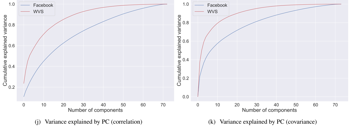
Figure S10: Variance explained by principal components. This figure shows the number of independent underlying factors behind the variation in our Facebook measure and compares it to the traditional values-based measure. Specifically, it shows the cumulative share of total variation in our Facebook measure and the values-based measure explained by principal components. Panel (a) plots explained variance after standardizing, i.e. using the correlation matrix. Panel (b) plots explained variance without standardizing, i.e. using the covariance matrix.
