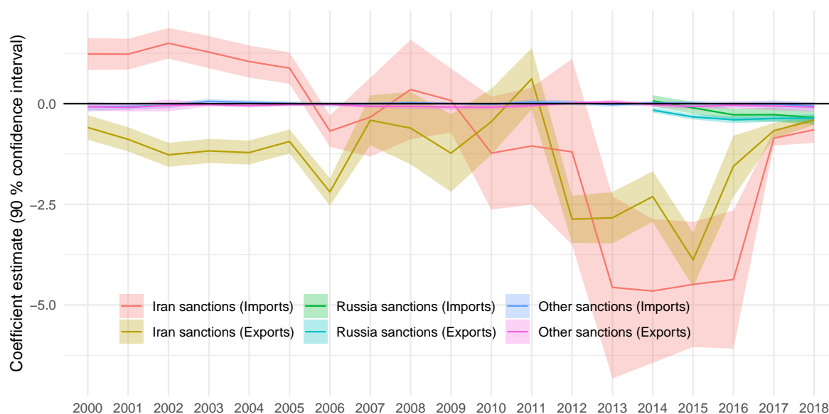
Figure 3: Coefficients from Gravity Estimation
