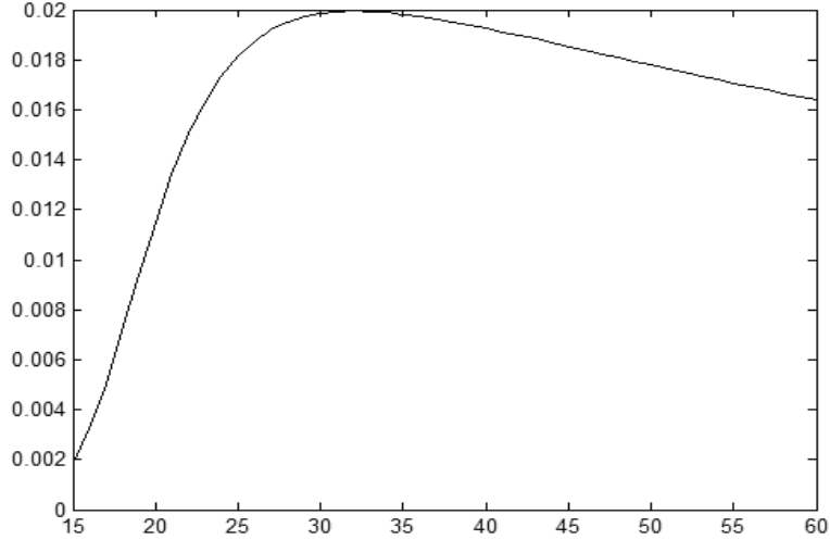
Figure 1: The function \psi(\bar{T}) defined in (3.4) for the parameters \eta_0 = 0.03 , s_0 = 1 , \theta_1 = 0.25 , \theta_2 = 0.5 and \theta_3 = 0.25 .
