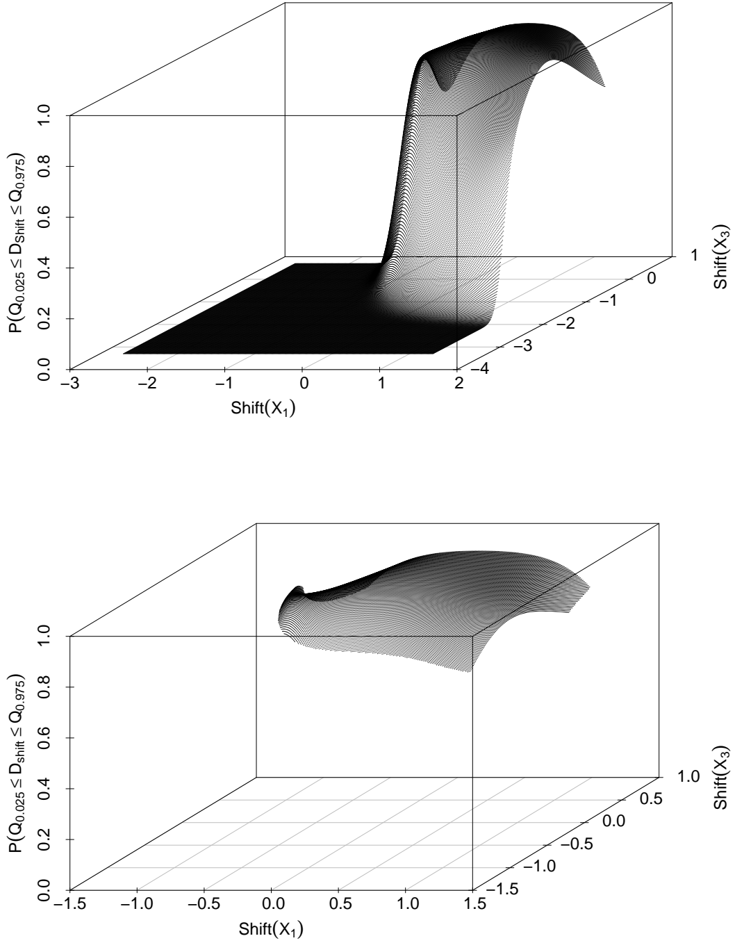
Figure 7: Probability that [Q_{0.025}, Q_{0.975}] covers the values of the DI when X_1 and X_3 are shifted; below: Same Surface with P(Q_{0.025} \leq D_{\text{shift}} \leq Q_{0.975}) \geq P_{\min} = 0.8 .
