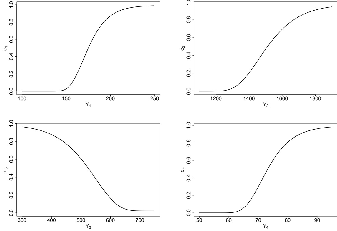
Figure 6: Desirability Functions of PICO Abrasion Index($Y_1$), 200%-Modulus ($Y_2$), Elongation at Break ($Y_3$) and Hardness ($Y_4$)
