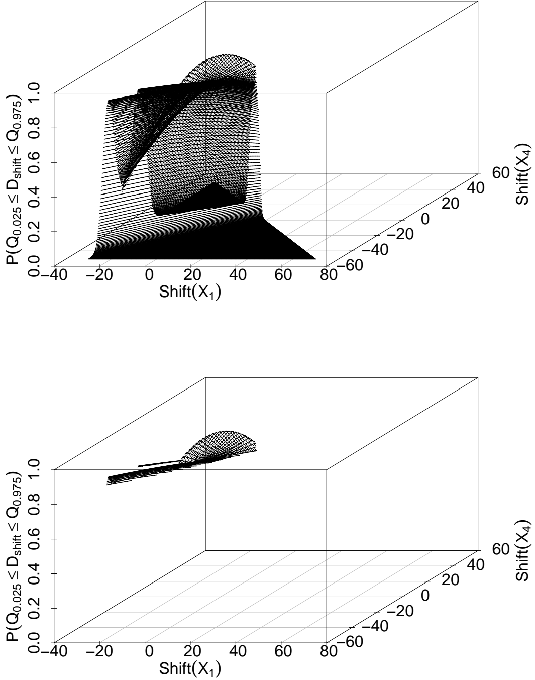
Figure 4: Probability that [Q_{0.025}, Q_{0.975}] covers the values of the DI when X_1 and X_4 are shifted; below: Same Surface with P(Q_{0.025} \leq D_{\text{shift}} \leq Q_{0.975}) \geq P_{\min} = 0.8 .
