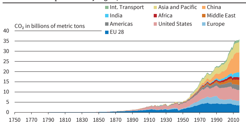
Figure 2 Annual World's CO 2 Emissions by Region, 1751–2017
