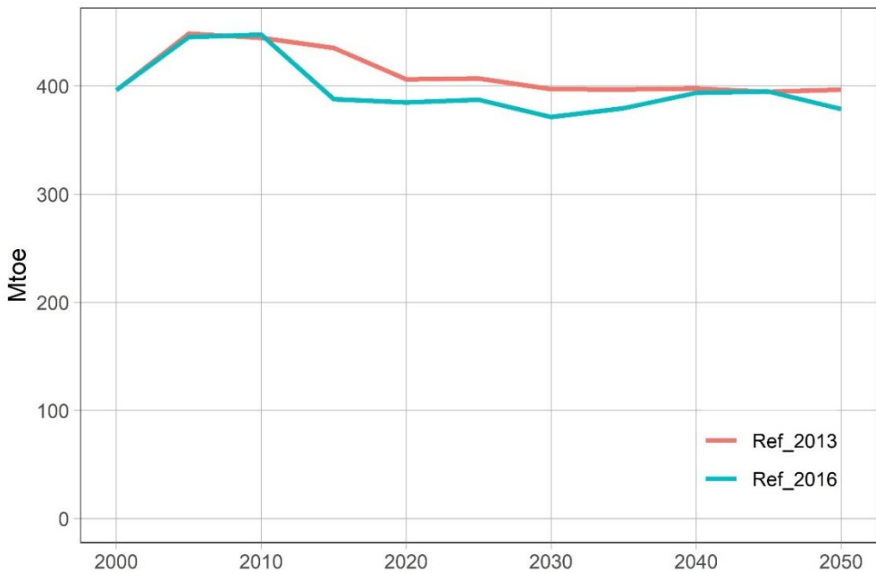
Figure 5: Fossil natural gas consumption in the European energy mix in the EU Reference Scenarios of 2013 and 2016.
