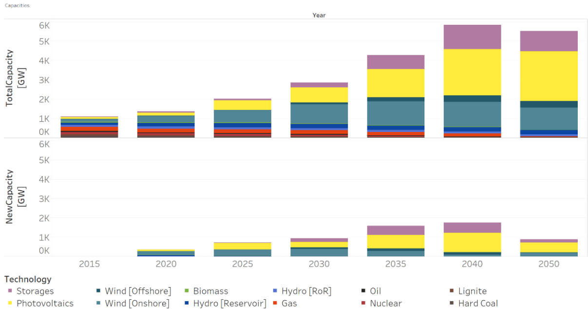
Figure 20: Electricity generation capacities Europe in the Paris-scenario until 2050.
