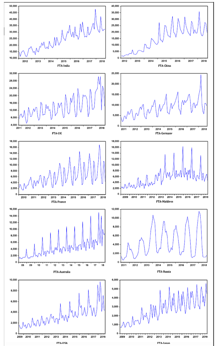
Figure 3: Time series plots of FTAs for the model estimation periods
