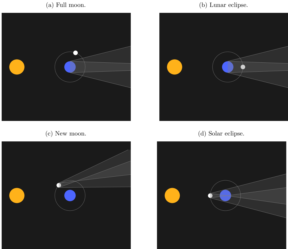
Figure 3: Eclipses, full moon and new moon.
