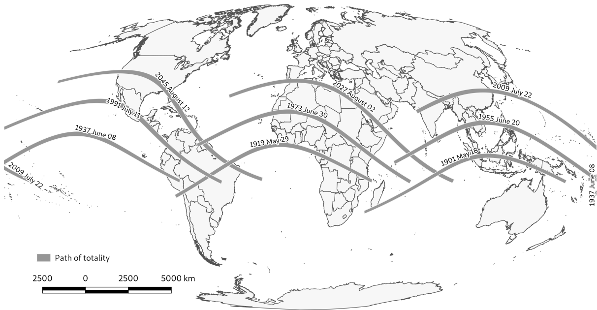
Figure 4: Eclipses from Saros 136.
