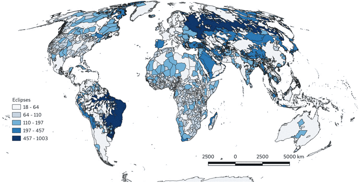
Figure 2: Distribution of total solar eclipses at the ethnic homeland level.
