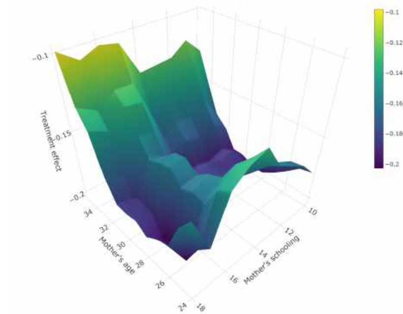
Figure 11 – Treatment effects of more than two children on worked for pay along the dimensions mother's education and mother's age (2SLS random forest)
