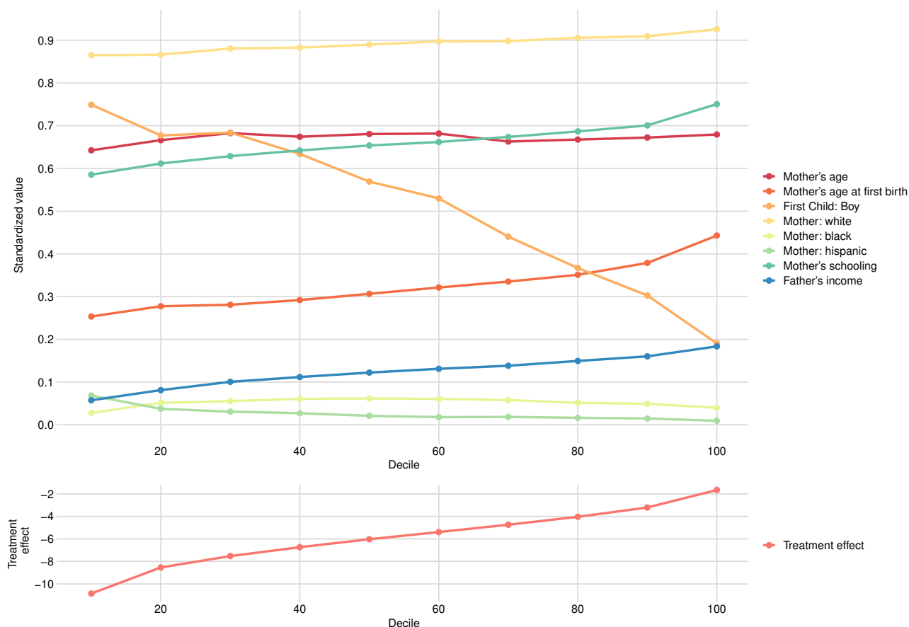
Figure 16 – Weeks worked: average values of covariates across different points of the treatment effect distribution
