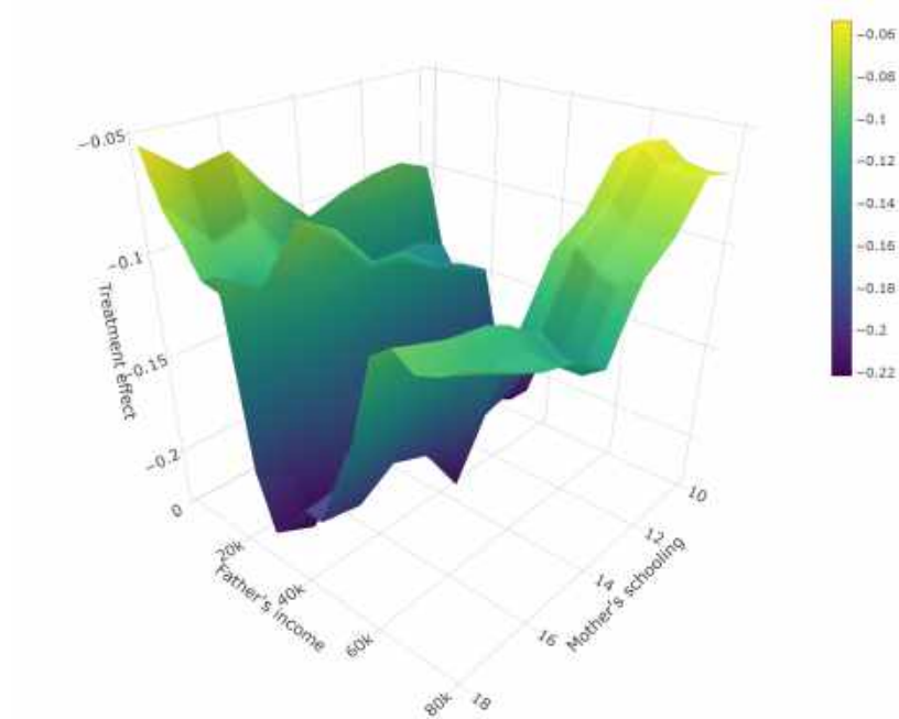
Figure 3 – Treatment effects of more than two children on worked for pay along the dimensions father's income and mother's education (2SLS random forest)
