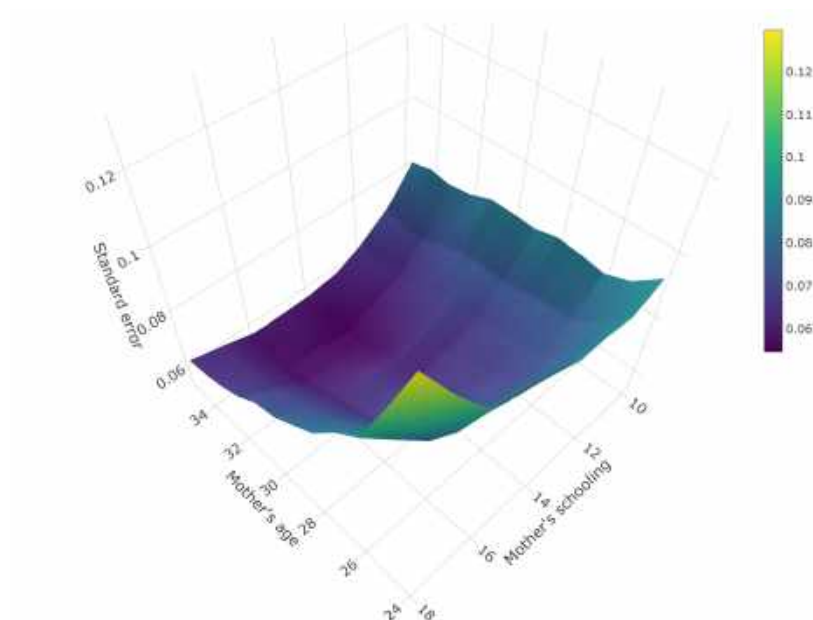
Figure 12 – Standard errors worked for pay along the dimensions mother's education vs. mother's age (2SLS random forest)
