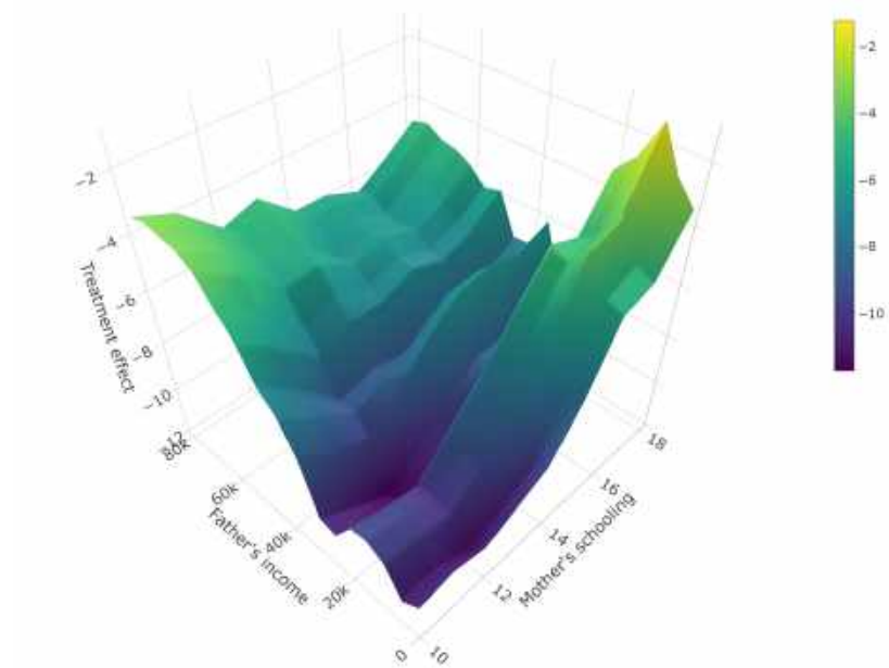
Figure 5 – Treatment effects of more than two children on weeks worked along the dimensions father's income and mother's education (2SLS random forest)
