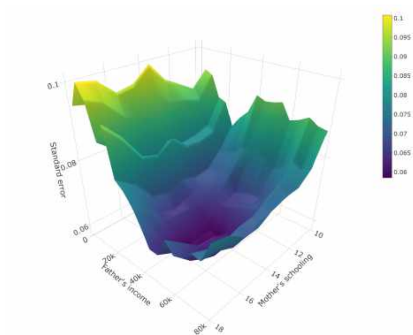
Figure 4 – Standard errors worked for pay along the dimensions father's income vs. mother's education (2SLS random forest)
