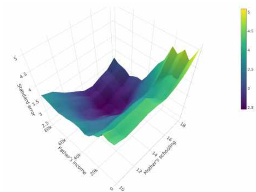
Figure 6 – Standard errors weeks worked along the dimensions father's income vs. mother's education (2SLS random forest)
