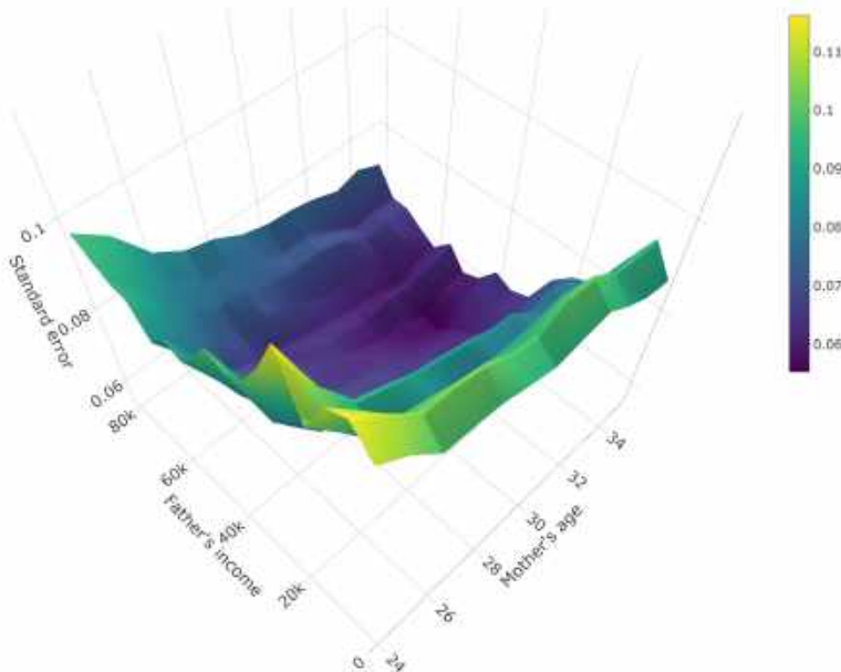
Figure 10 – Standard errors worked for pay along the dimensions father’s income vs. mother’s age (2SLS random forest)
