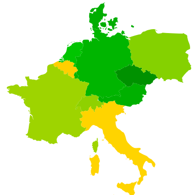
Neural Network
