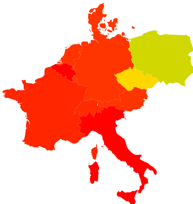
Naive
