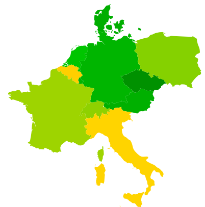
Neural Network
