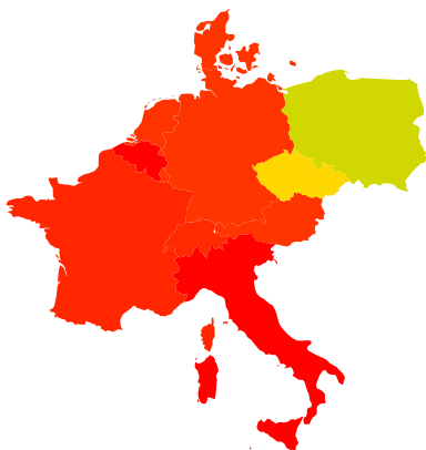
Naive
