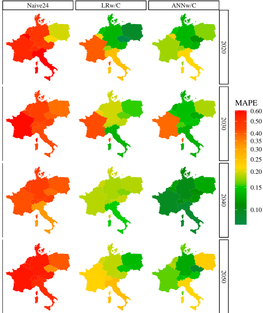
Figure 6: Mean absolute percentage errors (MAPEs) of the different price forecasting approaches in selected simulation years. The linear regression ( LRw/C ) and even more so the artificial neural network approach ( ANNw/C ) clearly outperform the persistence forecast ( Naive24 ). In contrast to the MAE, the MAPE accounts for the general increase of the price level (cf. Section 4.3) and therefore remains more stable over the course of the simulation.
