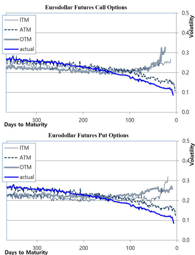
Figure 1. Actual and Implied Volatilities Using the Option Pricing Model in Eurodollar Futures and Futures Option Markets
