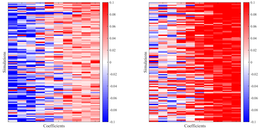
Figure 3: Difference between estimated and effective time variation for a_t for the FacTVP model (left panel) and the TVP-VAR (right panel). Coefficients appear in descending order of simulated time variation.
