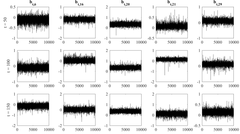
Figure 17: Markov chain for randomly selected elements of the coefficient vector b_t for different time periods.
