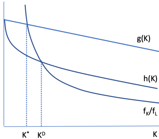
Figure 2: illustration of the proof of the position.
