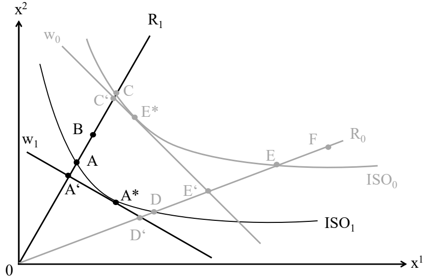
Figure 2 Illustration of the cost Malmquist index
