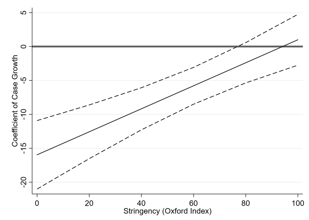
Figure 4: Interaction between case growth and stringency
