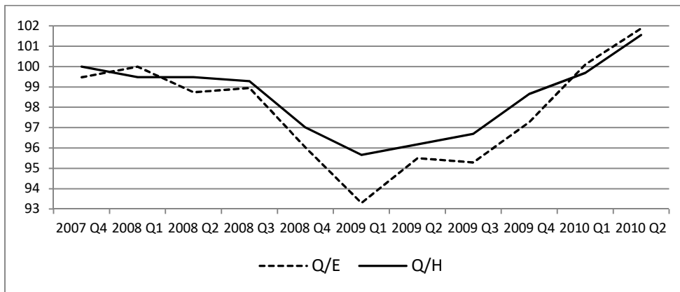
Figure 6 Indices of Q/E and Q/H for GR total manufacturing
