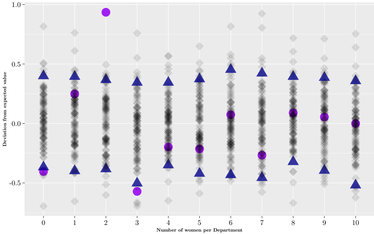
Figure 2: Top panel: Deviation from expected value summed over all disciplines. Bottom panel: Deviation from expected value summed over all disciplines, including bootstrapped 90% intervals.
