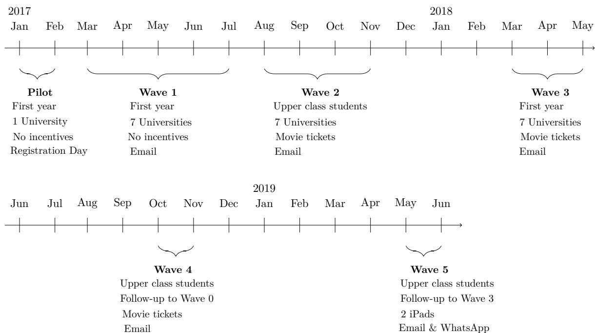
Figure 4: Survey timeline
