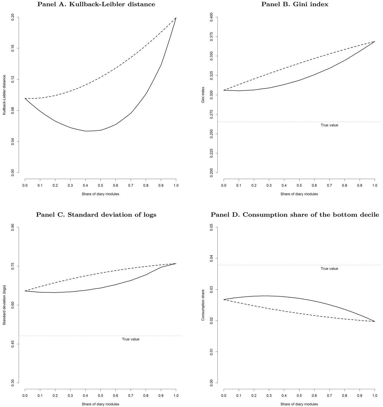
Figure 10: Optimal allocation of respondents to interview modes
