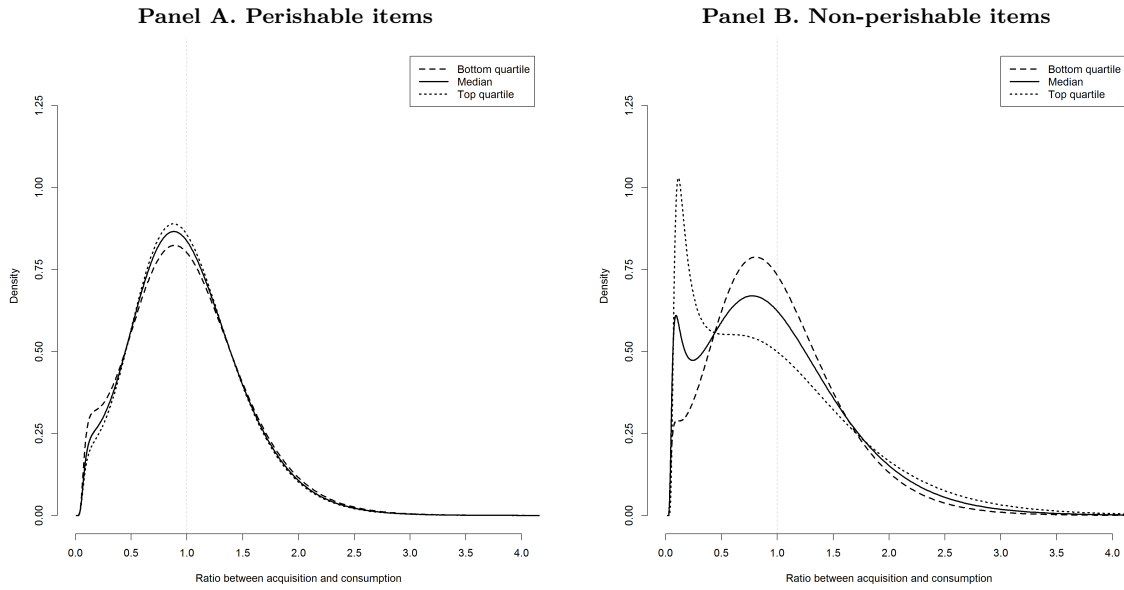
Figure 8: Survey errors in acquisition diaries and frequency of purchases
