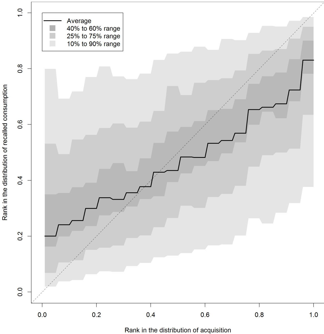
Figure 1: Household rank in diary and recall distributions
