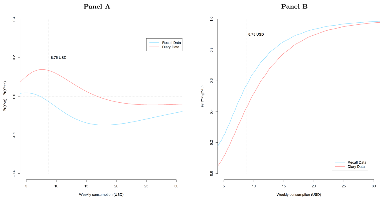
Figure 5: Poverty mismeasurement and the misclassification of households
