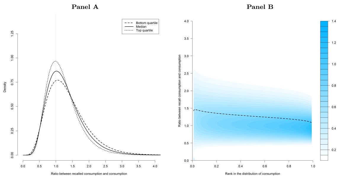
Figure 7: Survey errors in recalled consumption
