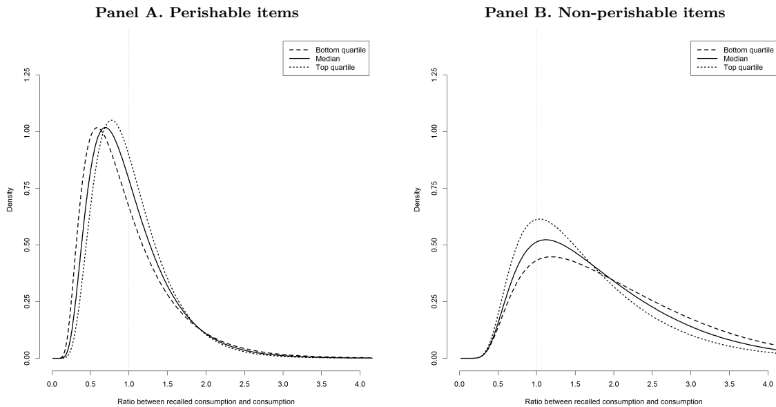
Figure 9: Survey errors in recalled consumption and frequency of purchases
