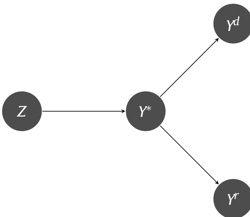
Figure 3: Directed acyclic graph of model assumptions
