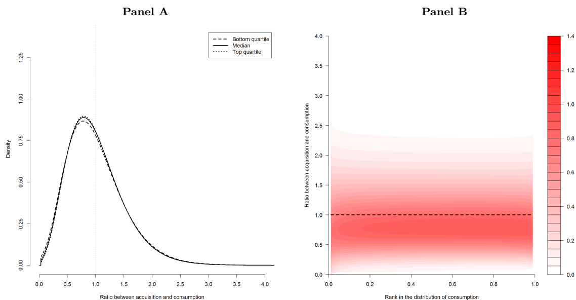
Figure 6: Survey errors in acquisition diaries
