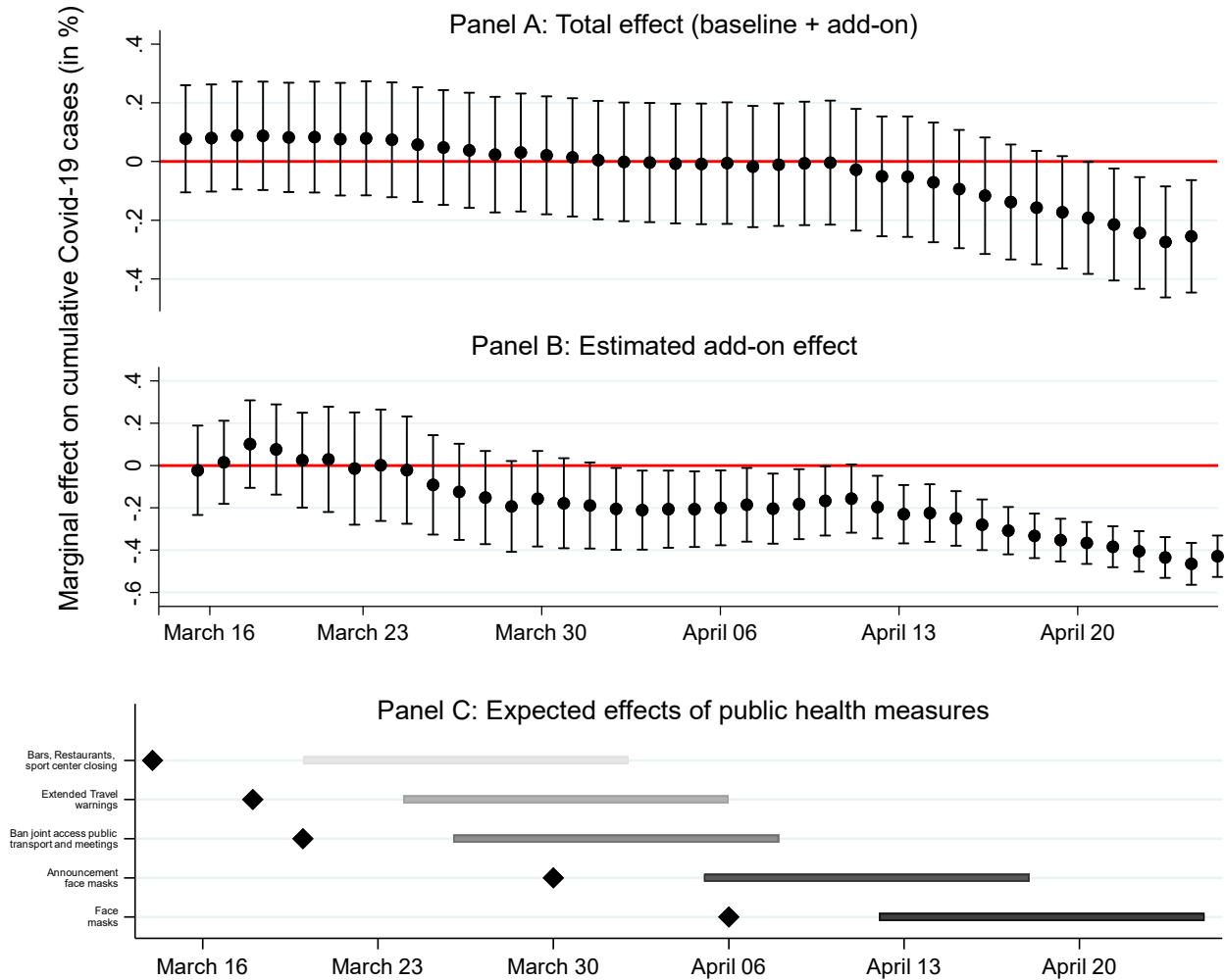
Figure 20: Estimated effects from incremental difference-in-difference (IDiD) model
