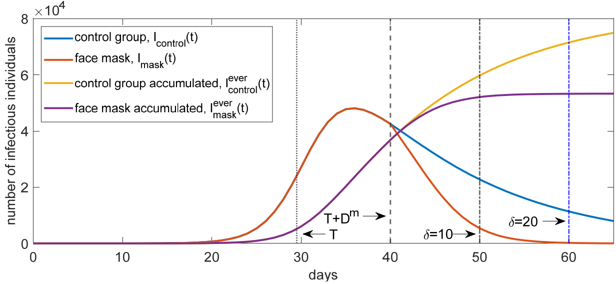
Figure 6: Theoretical effects of face masks on the number of infectious individuals I(t) and on the accumulated number of infectious individuals I^{\text{ever}}(t)
