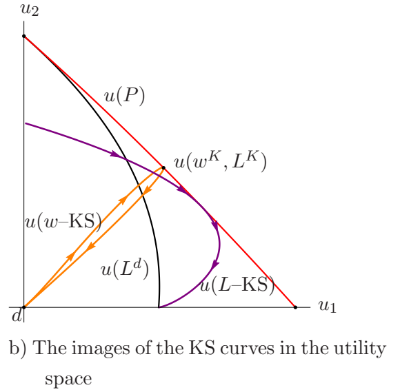
Figure 7: The solution curves for the KS-solution: the L -KS curve (purple) and the w -KS curve (orange) do not intersect on the Pareto curve (red).
