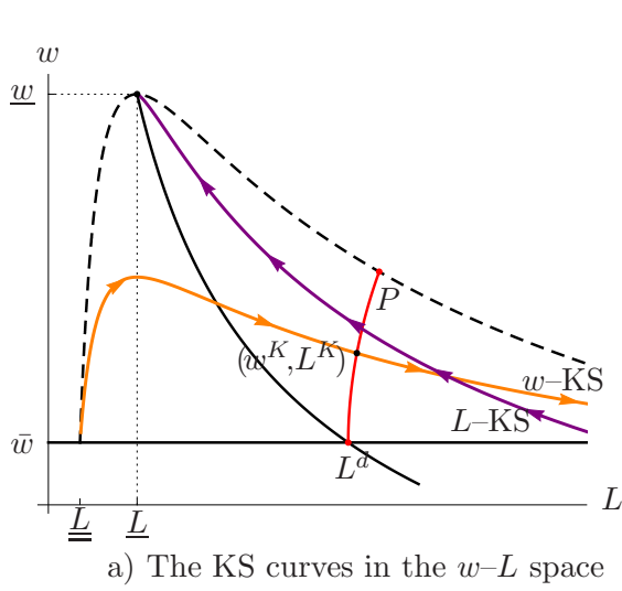
Figure 7: The solution curves for the KS-solution: the L -KS curve (purple) and the w -KS curve (orange) do not intersect on the Pareto curve (red).
