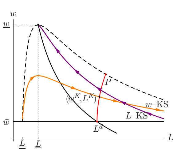
a) The KS curves in the w - L space
