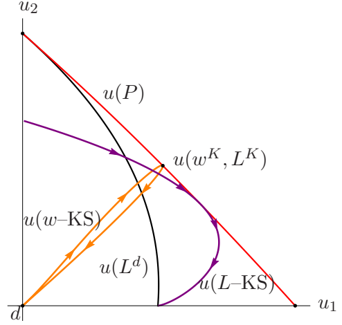
b) The images of the KS curves in the utility space
