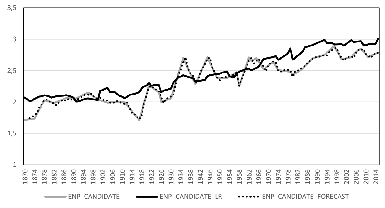
Figure 2 ARDL Model of ENP_Candidate
