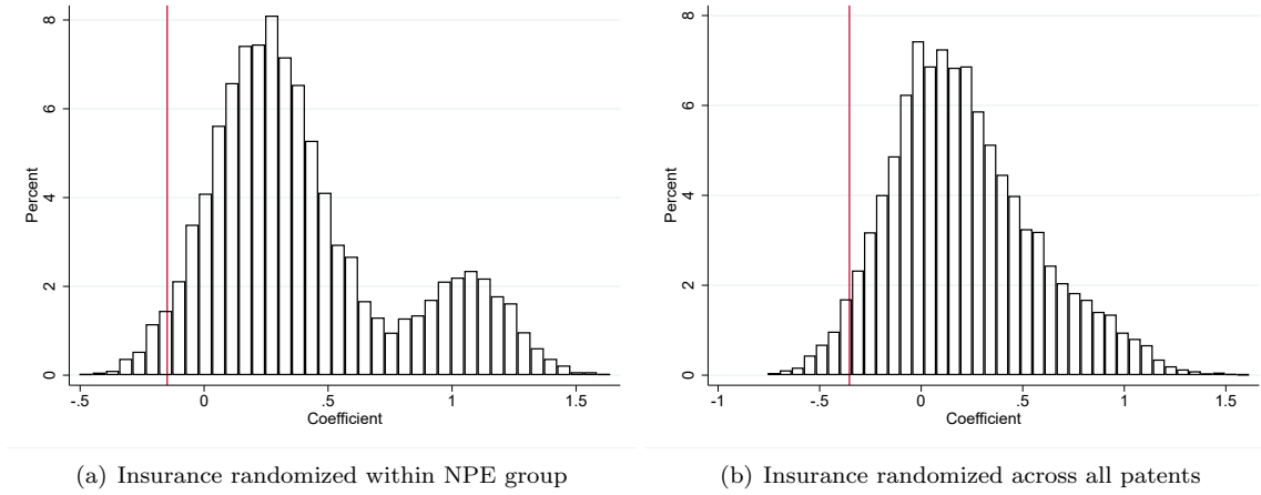
Figure A-4: Permutation Test
