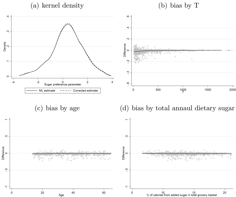
Figure 5.1: Sugar preference parameters
