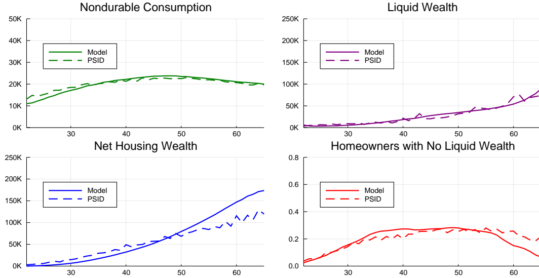
Figure 6: Fit of the Temptation Model
