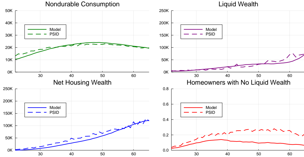
Figure 7: Fit of the Standard Model
