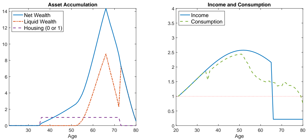
Figure 2: Lifecycle Profiles for Tempted Households
