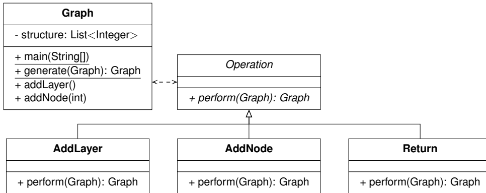
Figure 8: Representation of graph modification operations in a class structure for the purpose of non-deterministic choice.
