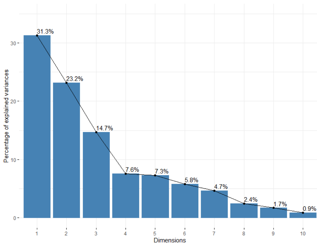
Figure A2. Scree plot of the principal component analysis
