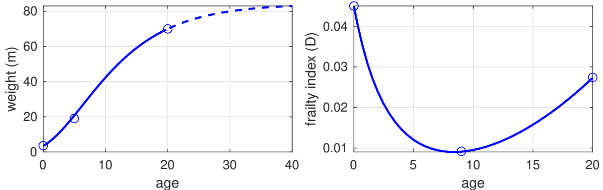
Left-hand side: solid line: calibrated model; dots: weight for age data for boys from CDC (2000); dashed line: hypothetical growth if growth were indeterminate. Right hand side: predicted frailty index; dots: constructed frailty index from mortality data.
