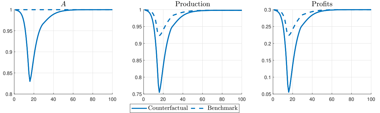
Figure 5: The dynamics of A , production, and profits
