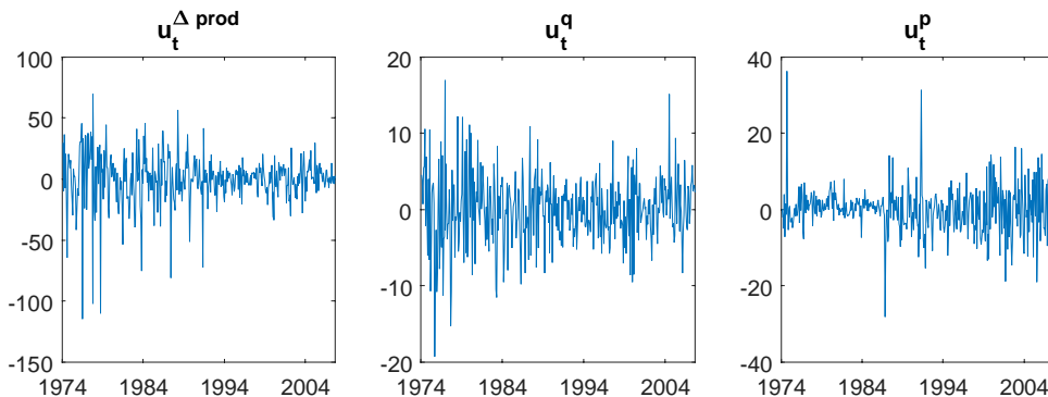
Figure 1: Reduced-form residuals of a plain VAR(3) model for the example data.
