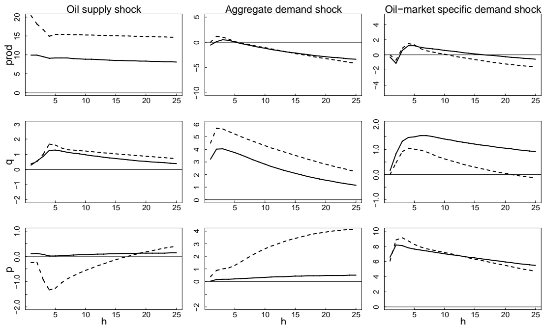
Figure 2: Comparison of impulse responses of plain VAR(3) (dashed line) and MS(3)-VAR(3) (solid line) model.
