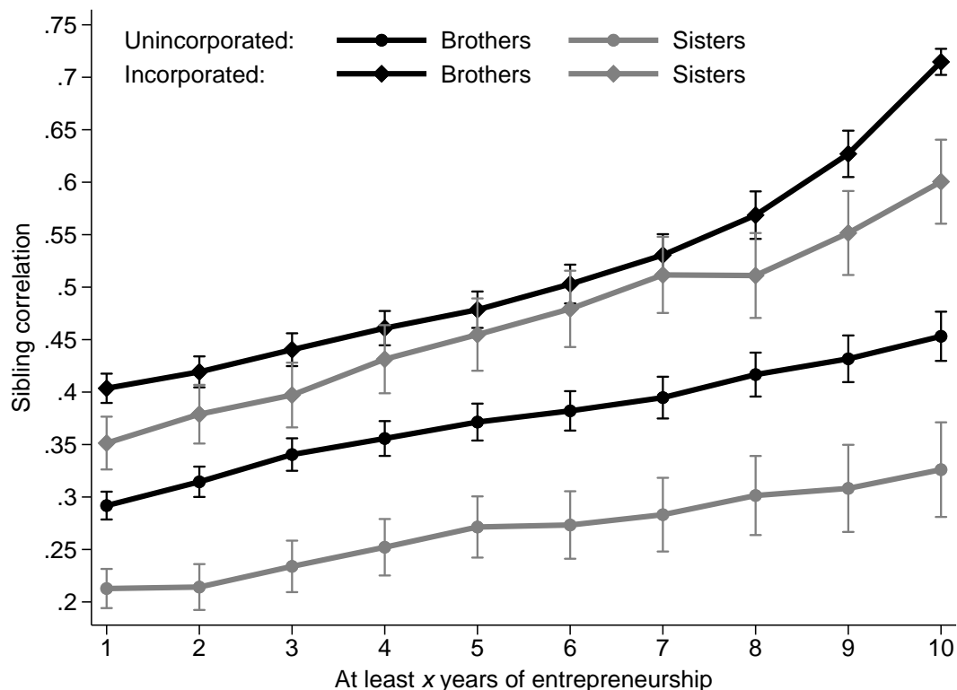
Figure 2.1: Sibling correlations in being a business owner for at least x years, separately by gender and type of business, with 95% confidence intervals.
