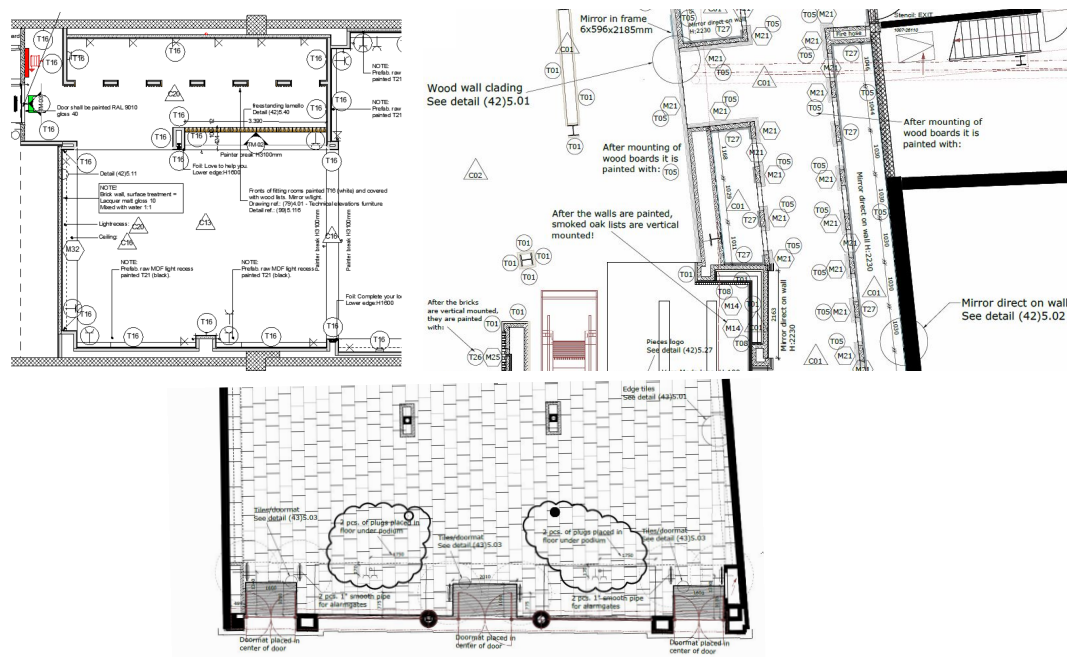
Illustration 1. Details of technical drawings for fashion stores.
