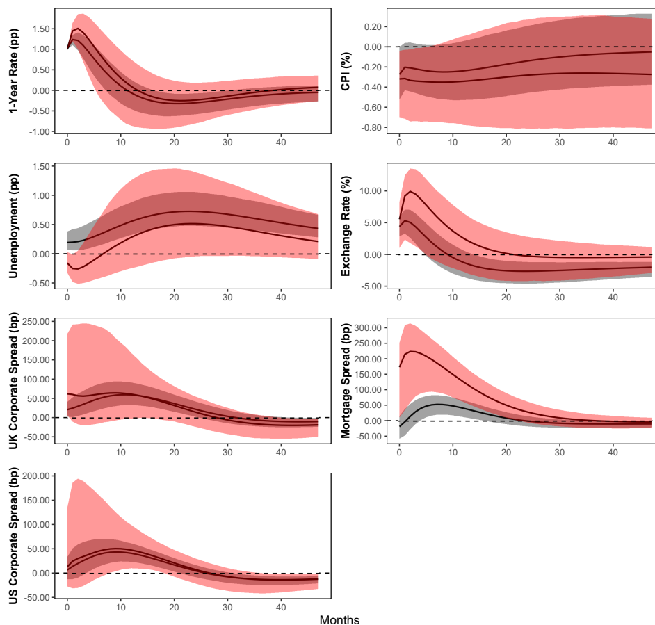
Figure A.1: Responses to a monetary policy shock with pointwise 68% confidence bands based on the moving-block-bootstrap methodology described in Jentsch and Lunsford (2019) using a block length of l = 4 . Grey areas indicate confidence intervals for the sample prior to the Great Recession from 1992m3-2008m8 and red areas represent confidence intervals for the period during and after the Great Recession from 2008m9-2015m1.
