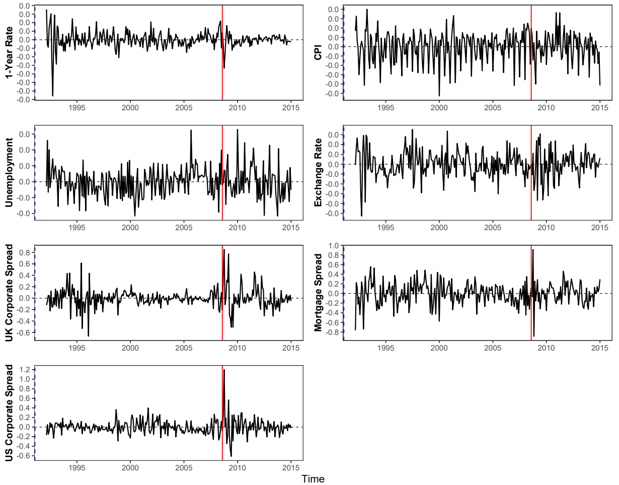
Figure 1: OLS residuals of UK monetary policy VAR(2) model. The solid red line indicates the variance break in August 2008 suggested by the likelihood based statistical criterion in (14).
