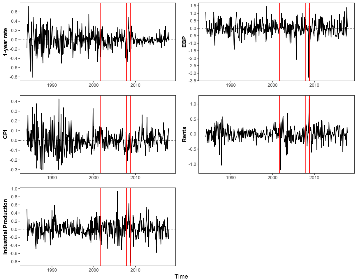
Figure 3: OLS residuals of US housing market VAR(12) model. The solid red lines indicate the three possible variance breaks in September 2001, November 2007, and November 2008 that are investigated.
