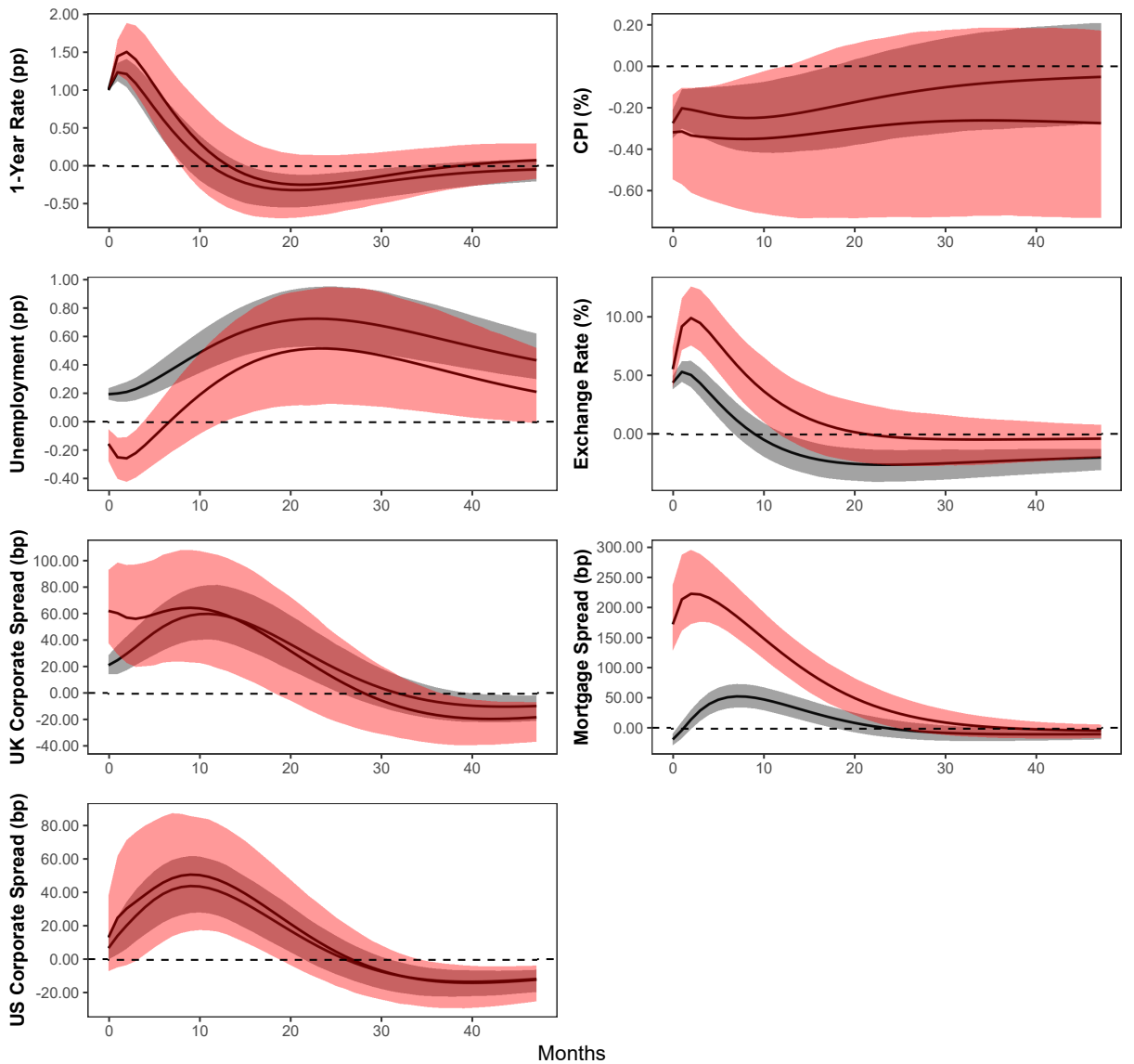
Figure 2: Responses to a monetary policy shock with pointwise 68% confidence bands based on a wild bootstrap. Grey areas indicate confidence intervals for the sample prior to the Great Recession from 1992m3-2008m8 and red areas represent confidence intervals for the the period during and after the Great Recession from 2008m9-2015m1.
