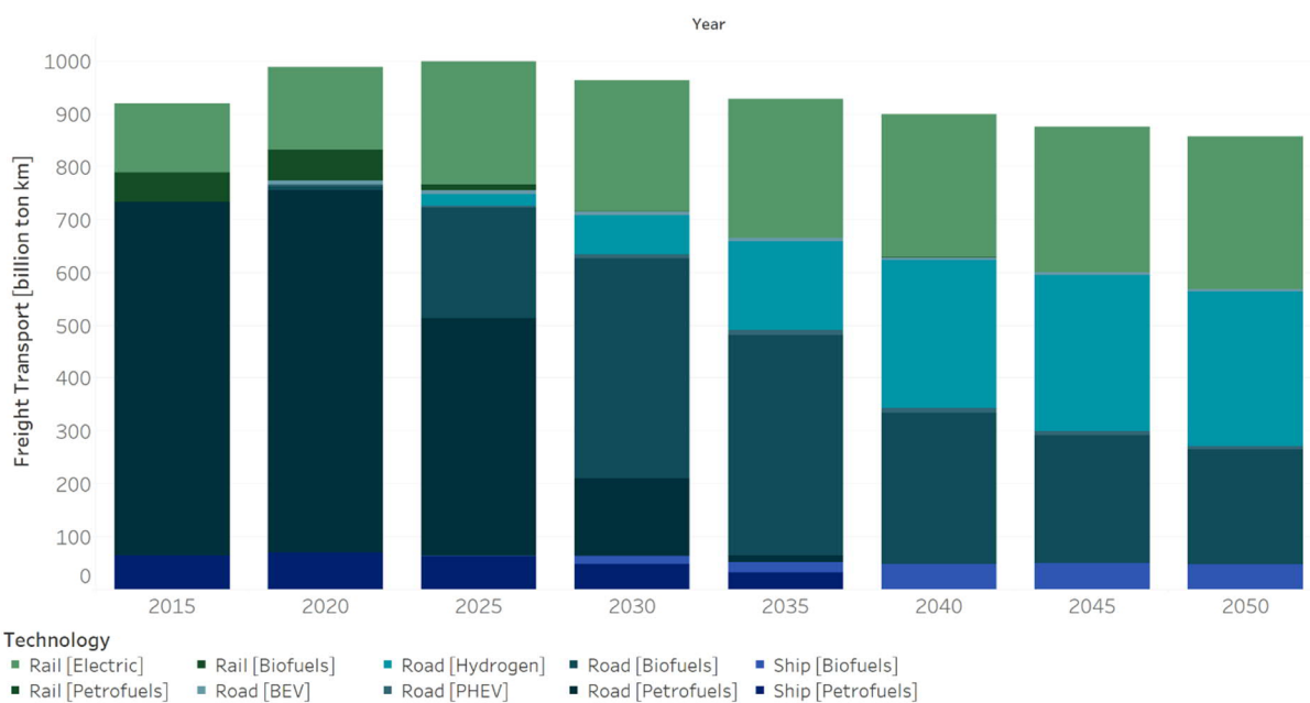
Figure 8: Energy demand for freight transport (until 2050, by technology and fuel)
