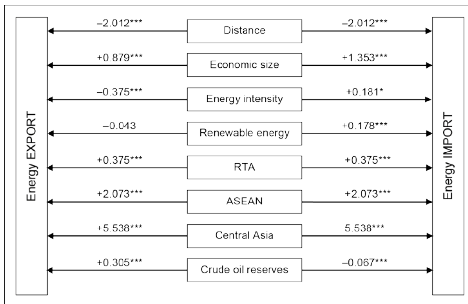
Figure 9: Results Overview
