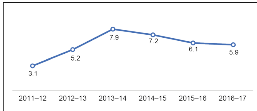
Figure 3: Applicability Dimension
