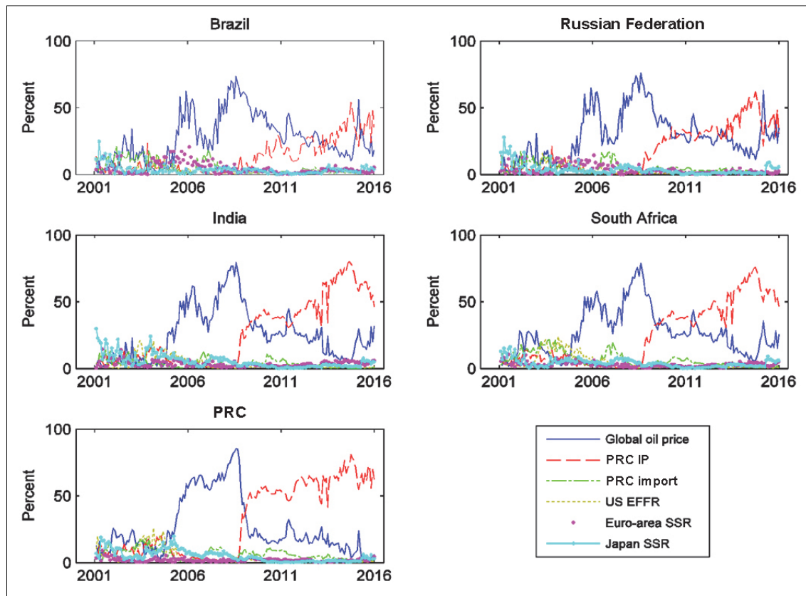
Figure 3: Time-varying Variance Decomposition (BRICS)
