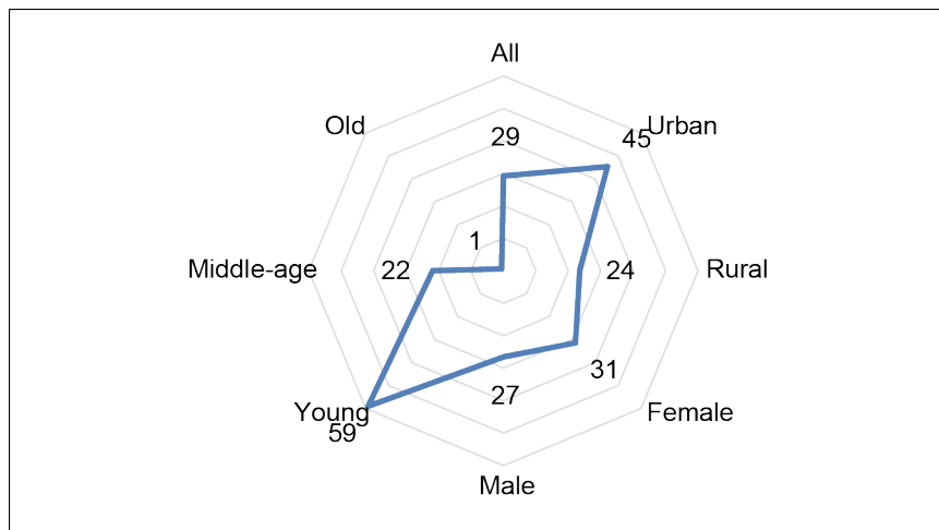
Figure 5: Internet Users
