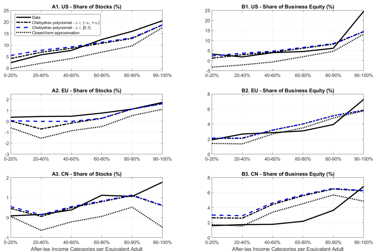
Figure E.2 – Calibration of the general version of the model with uninsurable labor-income risk ( \rho_{ys}^2 + \rho_{yb}^2 = 0.50 ). “CN” denotes China. All income categories are derived from actual data.
