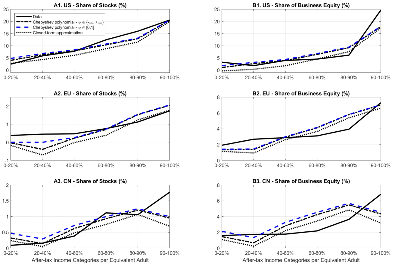
Figure 4 – Calibration of the general version of the model with uninsurable labor-income risk ( \rho_{y,s}^2 + \rho_{y,b}^2 = 0.75 ). “CN” denotes China. All income categories are derived from actual data.
