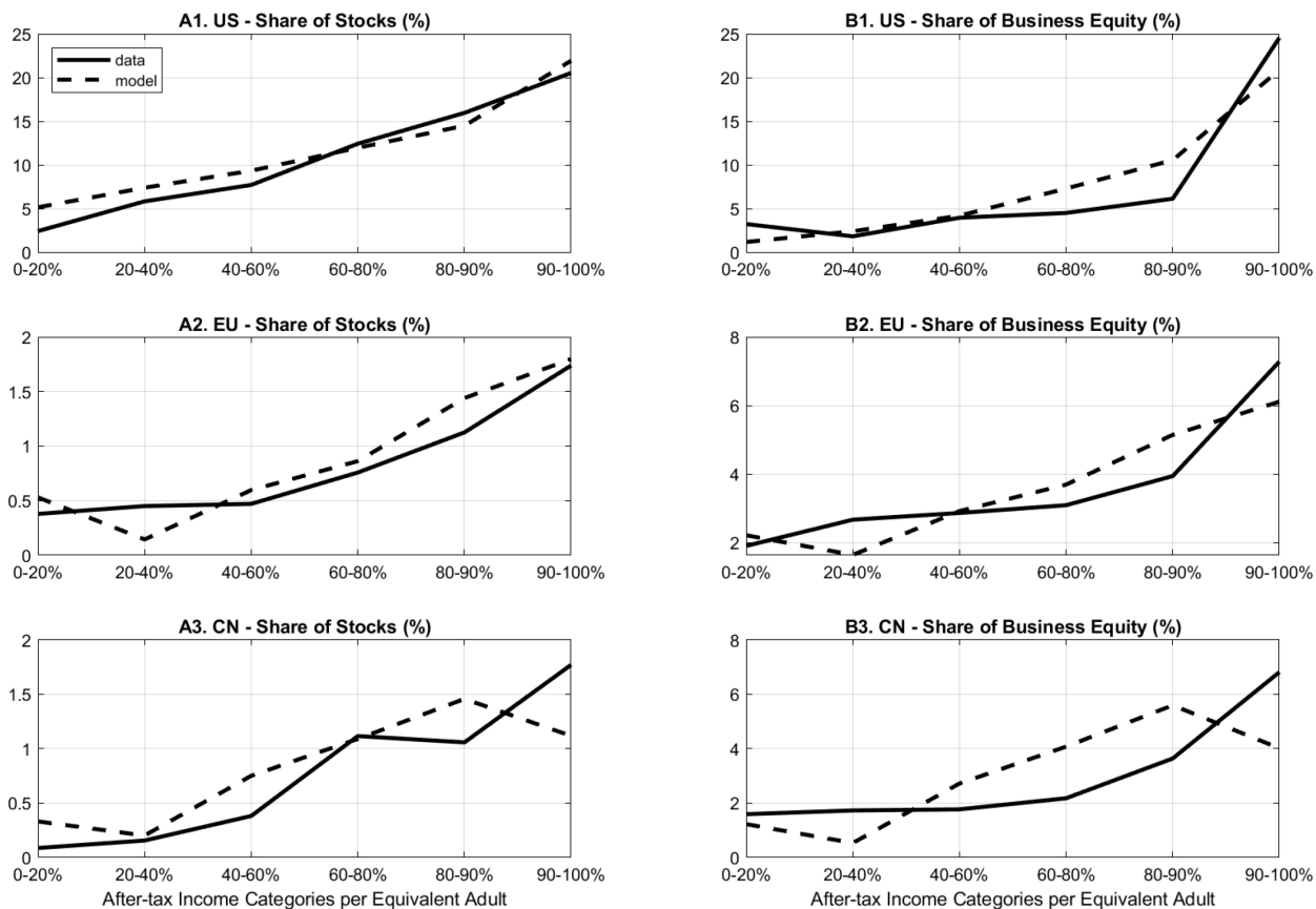
Figure 3 – Benchmark calibration of the special case of the model with insurable labor-income risk ( \rho_{y,s}^2 + \rho_{y,b}^2 = 1 ), using the closed-form solution. “CN” denotes China.
