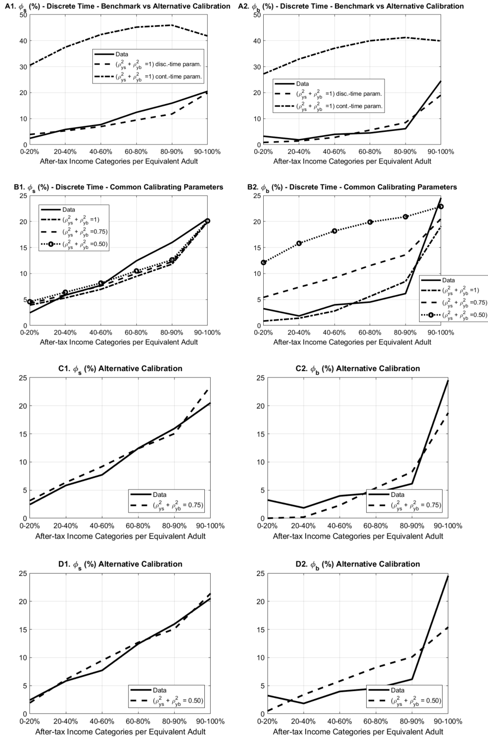
Figure F.1 US - Discrete-time numerical simulations, using exponential projection on the model with two risky assets. All income categories are derived from actual data.
