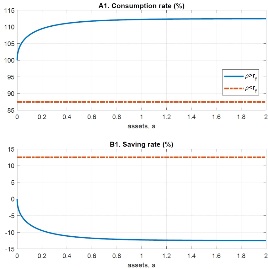
Figure O.A.1 Consumption rates and saving rates using the solution given by (A.64)
