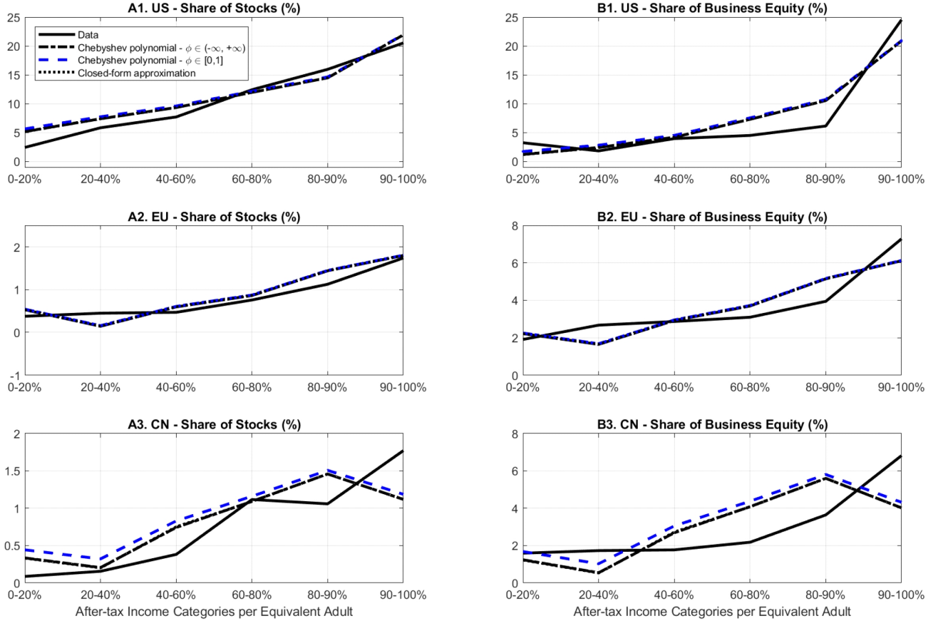
Figure E.1 – Demonstration of the small quantitative importance of short-selling constraints, in the version of the model with insurable labor-income risk ( \rho_{y,s}^2 + \rho_{y,b}^2 = 1 ).
