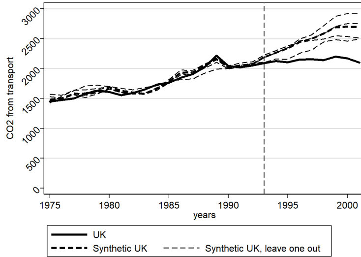
Figure 9: CO_2 from transport: Leave-one-out
