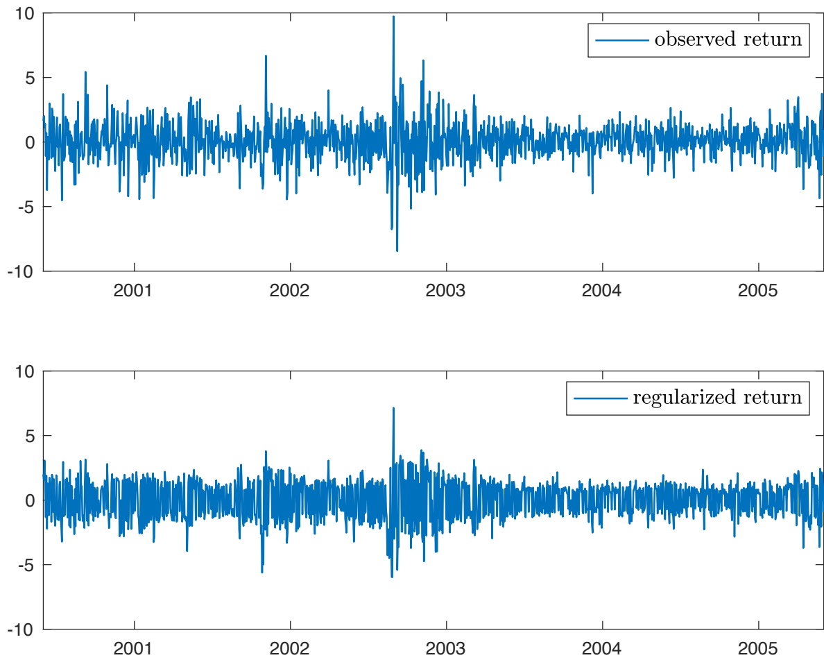
Figure 3: Observed returns and regularized returns (in percent) for a representative stock (Exxon Mobil Corporation) and period (4/19/2000–4/26/2005).
