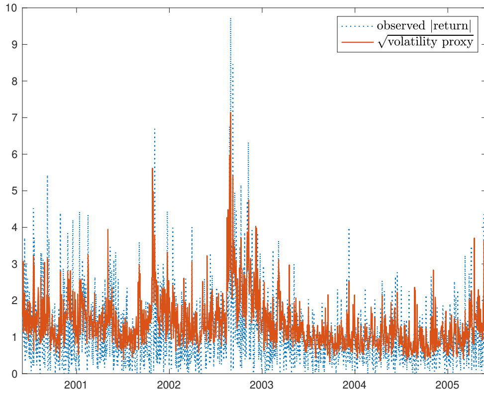
Figure 2: Observed absolute returns and the square root of the volatility proxies (in percent) for a representative stock (Exxon Mobil Corporation) and period (4/19/2000–4/26/2005) used to model the conditional univariate variances for DCC(-NL) respectively ID-DCC(-NL); see Equation (2.1) respectively Equation (3.1).
